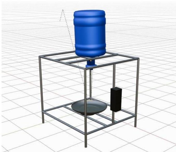
Gambar 1. Purwarupa smart feeder ikan lele berbasis IoT.
